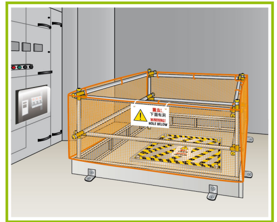
Provide guard-rails, toe-boards and warning signs at the floor opening
