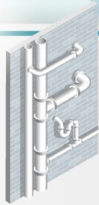
樓宇排水裝置 Building Drainage Installation
