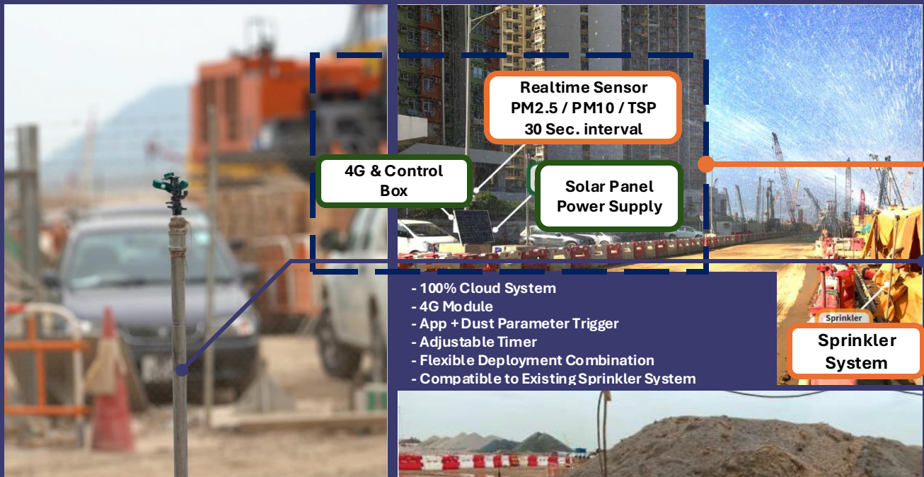
Automatic Sprinkler Head
