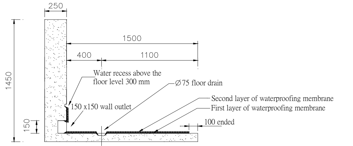
Sec B-B
