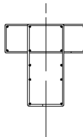
End View
