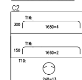
BAR BEND SCHEDULE
