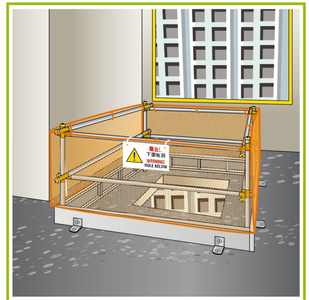
Provide guard-rails, toe-boards and warning signs at the floor opening.
