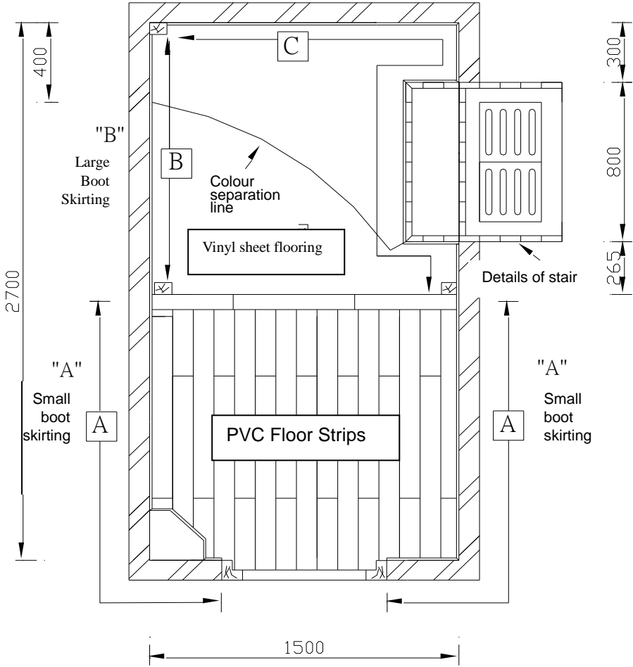
Layout Plan
