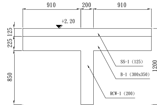
SECTIONAL VIEW B-B
