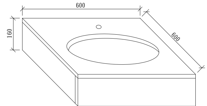
Basin Bench Top 3-D Plan
