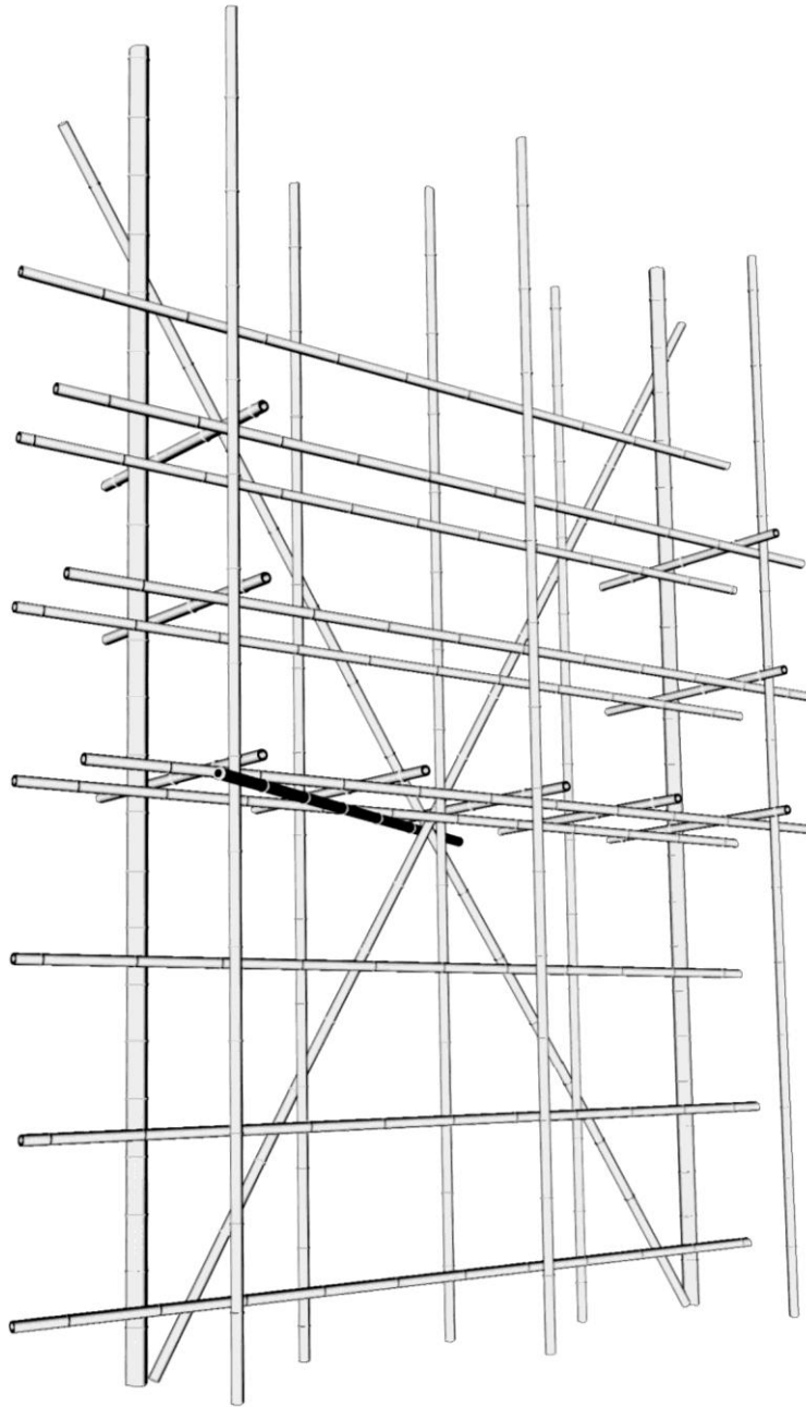
Combination of bamboo scaffold (Not to Scale)
