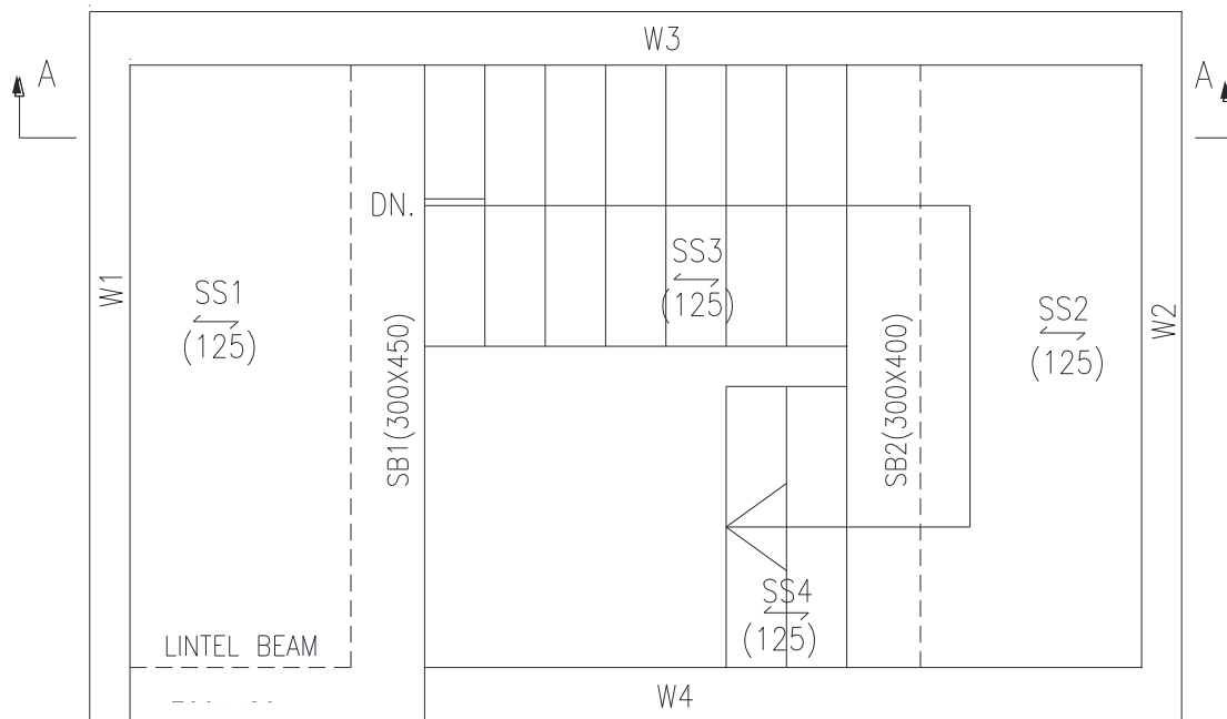
PLAN (1:30)
